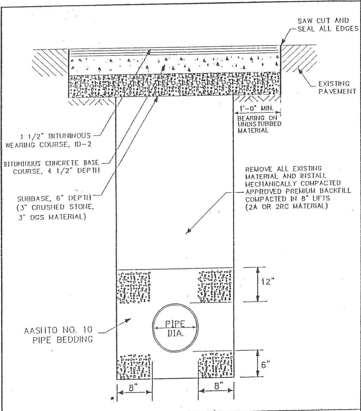
SPECIFICATIONS FOR STREET PAVEMENT REPLACEMENT DETAIL
